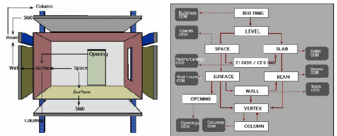
Figure 4: The architectural and structural views afforded by the PDB.
