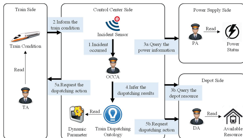
Figure 1: Architecture of the OMA-HSR
