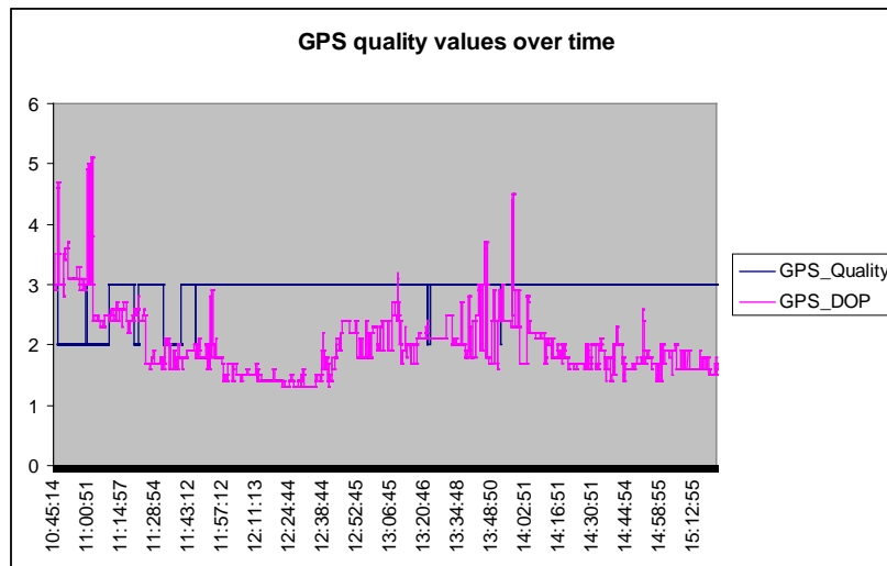
Figure 9. RTK GPS functioning near high buildings.
